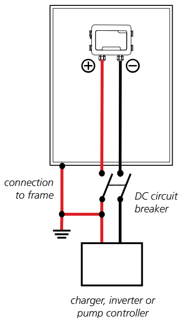
Figure 4a: Connecting a single module
